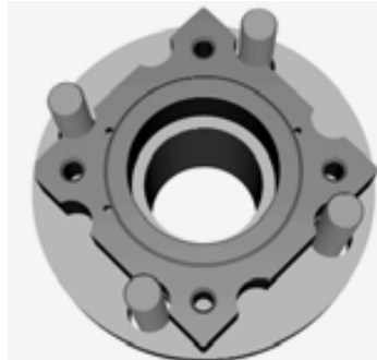
Figure 3 SRB-7RS™ Safety Head Companion Flange Bolting Pattern (Capscrews removed for clarity)
